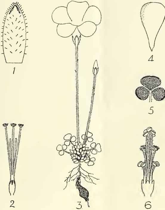
FIG. 3. Oxalis Fergusonae , Salter. 1. Sepal \times 8 . 2. Gynaecium \times 5 . 3. Plant \times 1\frac{1}{2} . 4. Petal \times 1\frac{1}{2} . 5. Leaf (dry) \times 4 . 6. Androecium \times 5 . ( Bolus Herb. 20176.) Del. T. M. Salter.
